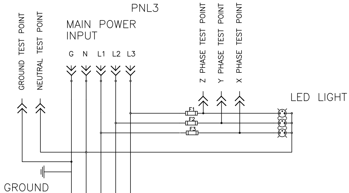
BRANCH POWER PNL1 19 PIN 6 CIRCUIT 208V
