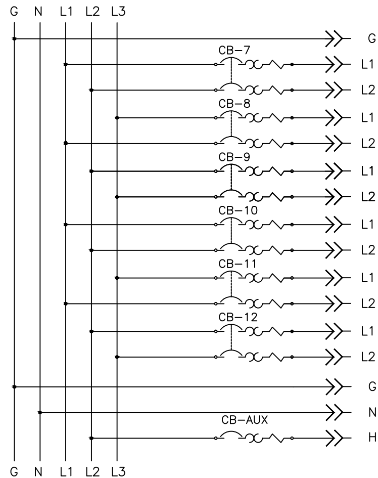
BRANCH POWER PNL2 Connector AUX 125V 2P3W 20AMP
